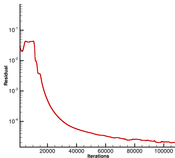
Figure 2.22: Convergence of residual for test case 2.4.4
