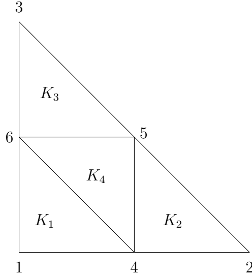
Figure 3.1: Subdivided triangle K .
