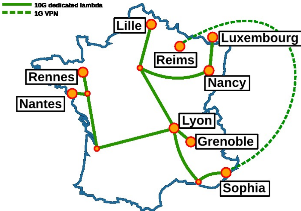
Figure 3.3: GRID'5000
