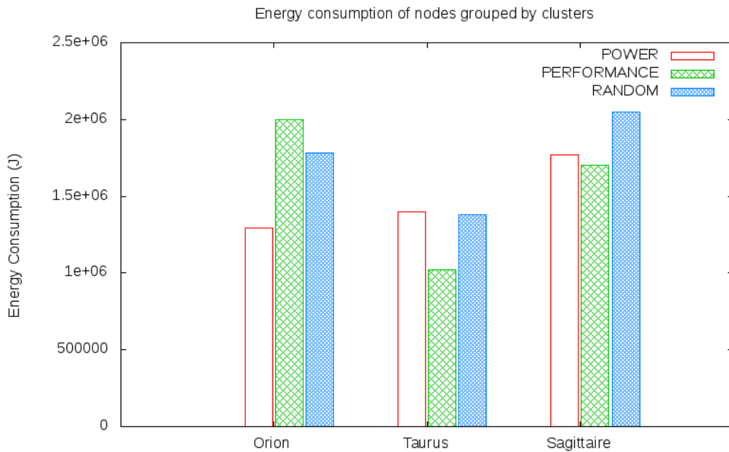
Figure 3.9: Cumulated energy consumption per cluster under POWER, PERFORMANCE and RANDOM scheduling policies.
