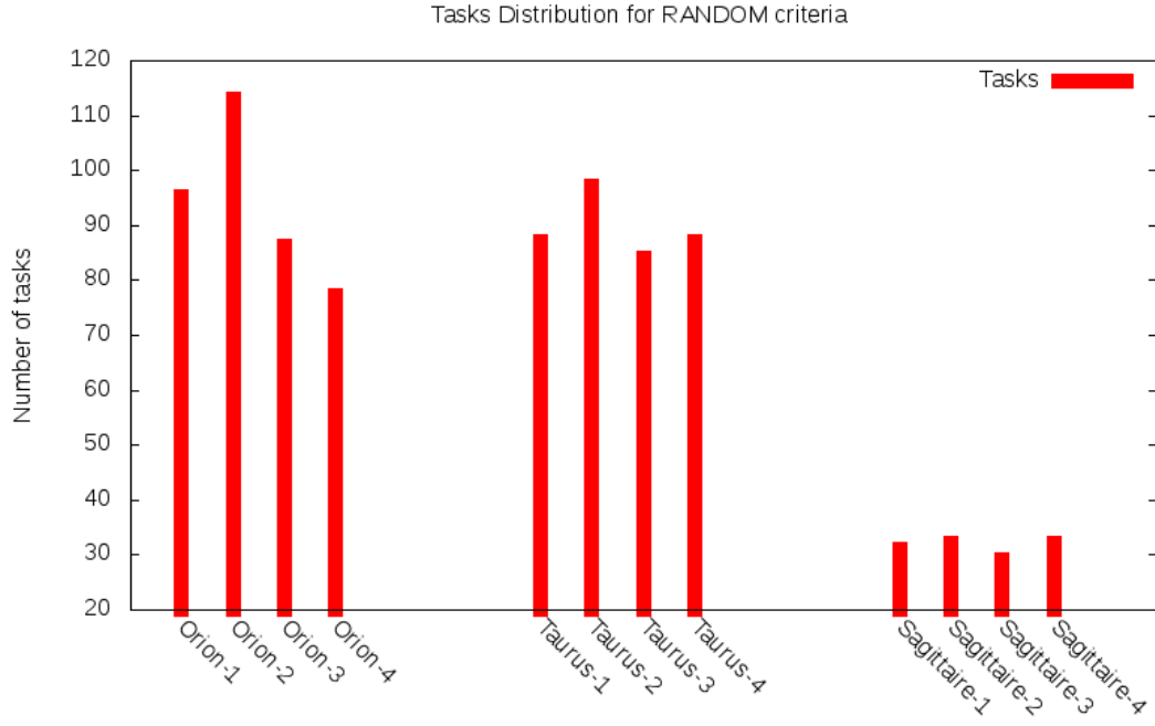
Figure 3.8: Tasks distribution with random placement.
