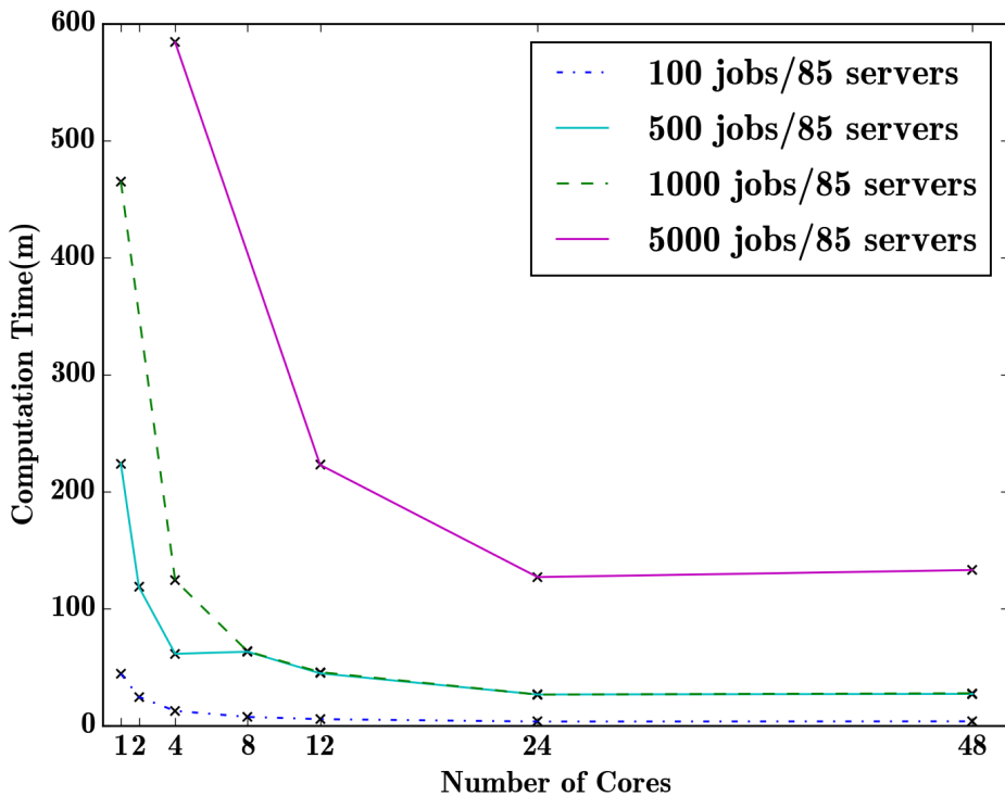
Figure 4.6: NSDE-2 execution time for generating mapping solutions related to 4 datasets and 111 servers
