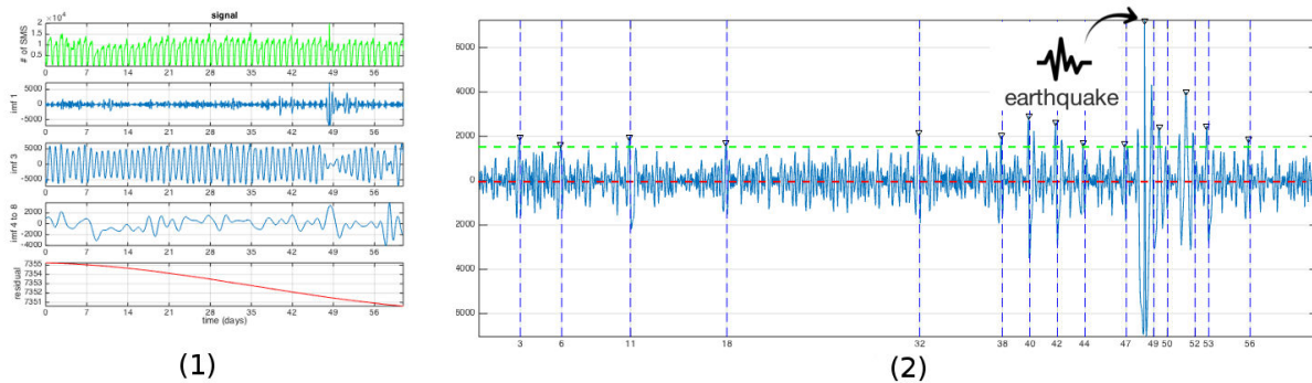
Figure 4.2.3: (1) EMD of the original temporal signal: number of SMS sent per day. One can clearly identify a day oscillation in the IMF 3. IMF 1 is high frequency variation and other IMF (4 to 8) are low frequencies, (2) For IMF 1, the high frequency of EMD is linked to specific events, the earthquake on the 18th April 2014 induces a perturbation on that mode. The red line corresponds to the mean.
