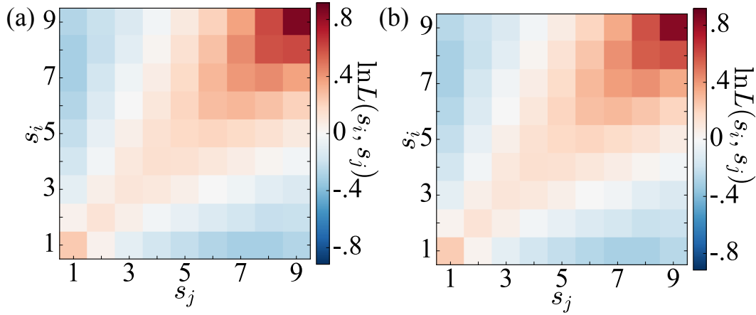
Figure A.1.2: L(s_i, s_j) normalised socioeconomic class connectivity matrices in case of two null models (for definition see Eq. 6.1 in the main text). In each case the numerator was taken as the socioeconomic class connectivity matrices of the original network, while the denominator was measured from a null model structure of (a) NM1, (b) NM2.
