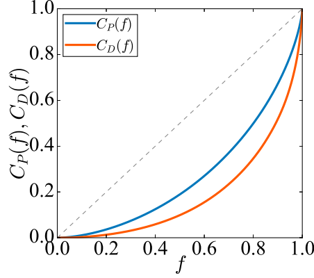
Figure 5.2.1: Pareto principle. Cumulative distributions of P_u (blue line) and D_u (orange line) as functions of sorted fraction f of individuals. Dashed line shows the case of the perfectly balanced distribution.
