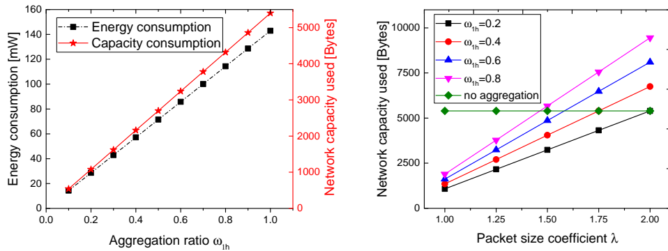
(a) Energy and network capacity with different \omega_{1h} (here \lambda_{1h} = 1 ). (b) Network capacity with different \omega_{1h} and \lambda_{1h} .
