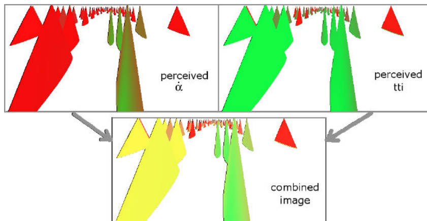
Figure 2.4 The Optical flow used in the vision based model [OPOD10] with the risk of collision that is a combination of the derivative of the bearing angle, to check for collision, and the Time To Interaction, to check for the imminence of the danger.
