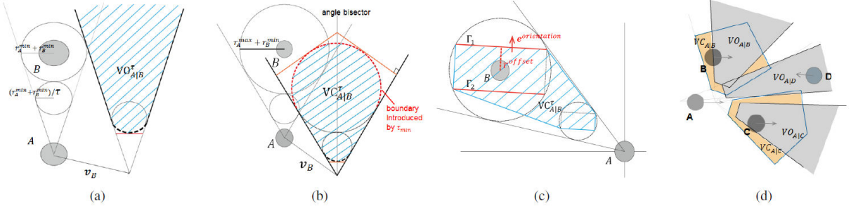
Figure A.3 (a) The velocity obstacle VO_{A|B}^\tau of an agent B to agent A is a truncated cone in the velocity space. (b) The velocity connection VC_{A|B}^\tau of an agent B to agent A contains the velocities that result in grouping A and B together for at least \tau_{min} seconds before time \tau . Here \tau_{min} = 1 . (c) VC_{A|B}^\tau for a rectangular constraint. (d) A situation where not all velocity constraints can be satisfied since VC_{A|B}^\tau \cap VC_{A|C}^\tau = \emptyset (group neighbors B and C are not close to each other). In this case, agent A tries to stay close to both B and C.
