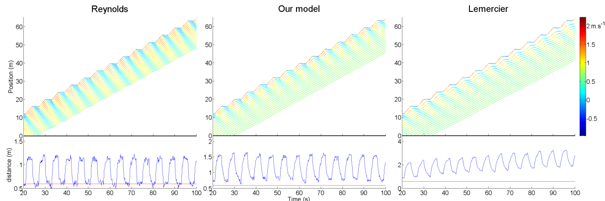
Figure 3.10 Simulations of agents following a leader with a rectangular signal speed with some noise. Reynolds: in Reynolds’s model there is no security distance, the agent can be closer to the leader than the desired distance leading to collision risk. Middle: in our model the followers keep close to the leaders with a security margin to prevent getting closer than a fixed distance. Right: in Lemercier’s model the following distance increases over time.
