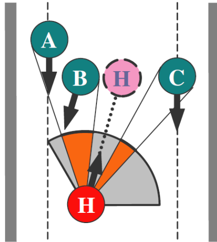
Figure 2.5 A rule, from the ruled-based algorithm proposed by [ST05], that defines a global strategy to avoid several agents at once in a corridor: pedestrian H searches for a safe direction interval when confronted by oncoming traffic.
