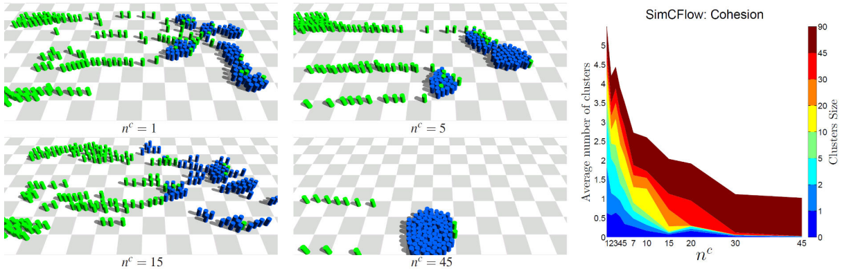
Figure A.4 Simulation results of a group (in blue) going through a crowd of individuals (in green) for different value of n^c . The simulations demonstrate that the group is more and more bound together and is less likely to break into small clusters with higher value of n^c , which is quantitatively confirm by the graph on the right.
