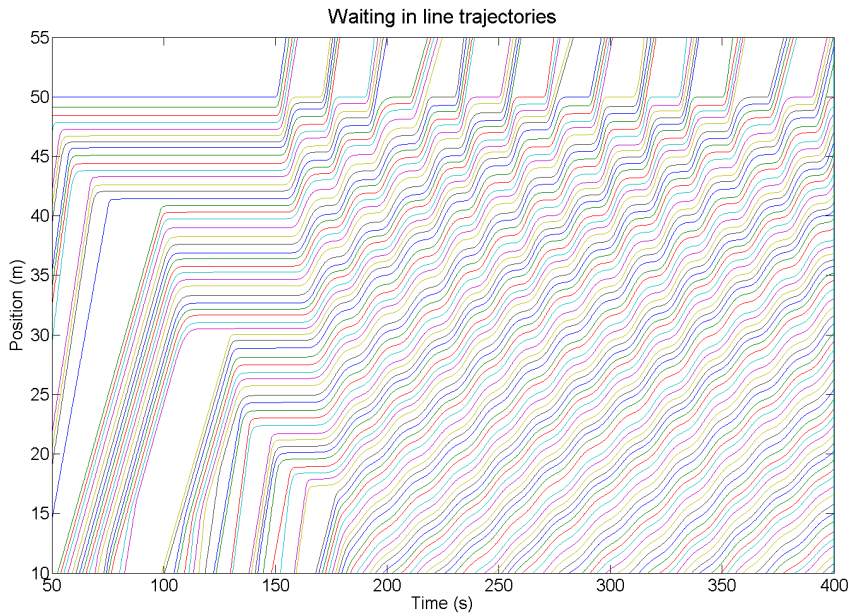
Figure 3.4 Trajectories of people lining up and waiting. Stop-and-go waves are created and propagated when the first walker in the line moves.
