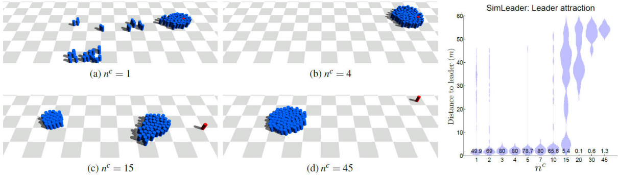
Figure A.6 Simulation of a leader (in red) trying to move a whole group (in blue) toward its goal. Different level of n^c were tested showing that an average level of cohesion is require, from the group, to move a whole group. The graph shows the distribution of the agents through the distance from the leader at the end of the simulation.
