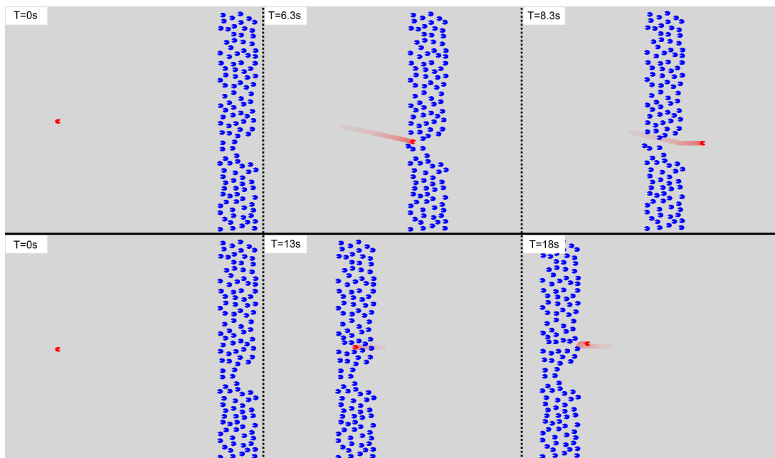
Figure 4.12 Simulation of an agent (in red) going through a flow that goes in the opposite direction. The flow has no tunnel but a section of it has a lower density. At the top, we have the simulation with EACS and at the bottom the simulation without EACS.
