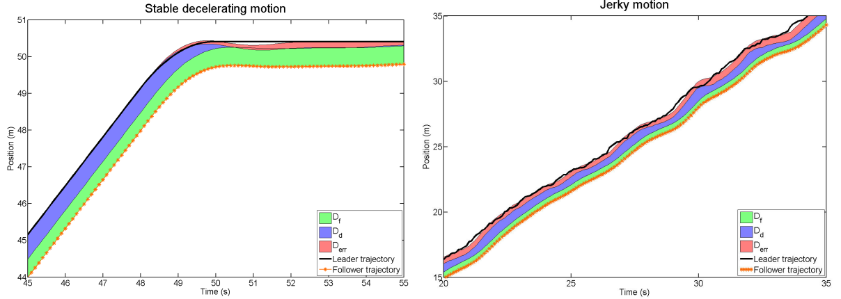
Figure 3.3 Visualization of the following distance computed for a leader with very stable motion (left) or with jerky motion (right).
