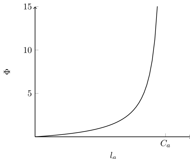
Figure 4.3: Kleinrock function.
