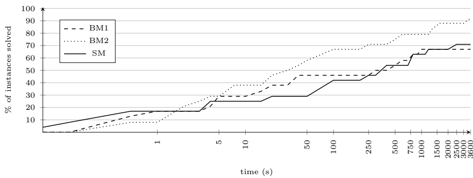
Figure 4.12: PUMF, T_2 : performance profile of MIP solving times (s).
