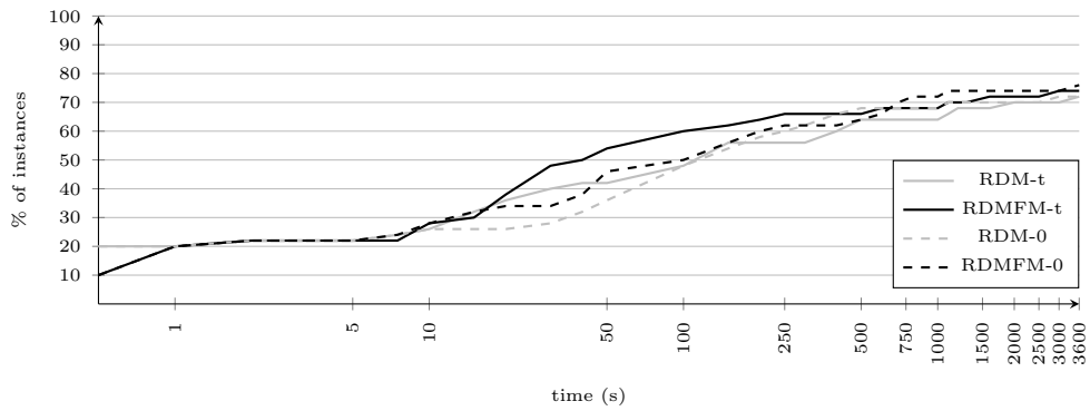
Figure 3.17: COCMST & TE-MSTP decision, T_{rand} : performance profile of the time (s) it takes to prove infeasibility, for \epsilon = -0.05 .
