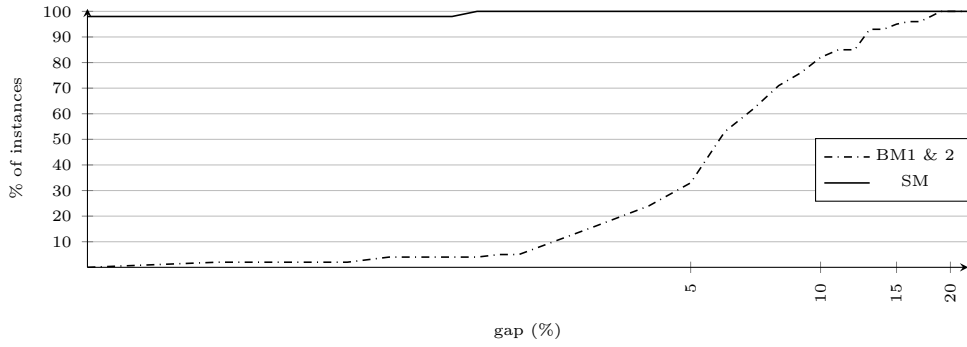
Figure 4.4: PUMF, T_1 : performance profile of Gap_{LP} (%).
