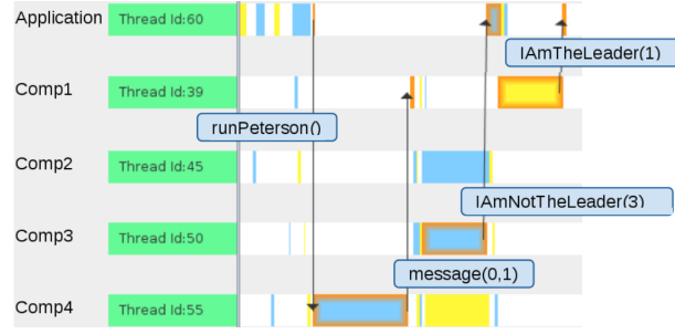
Figure 5.16 – Code execution
