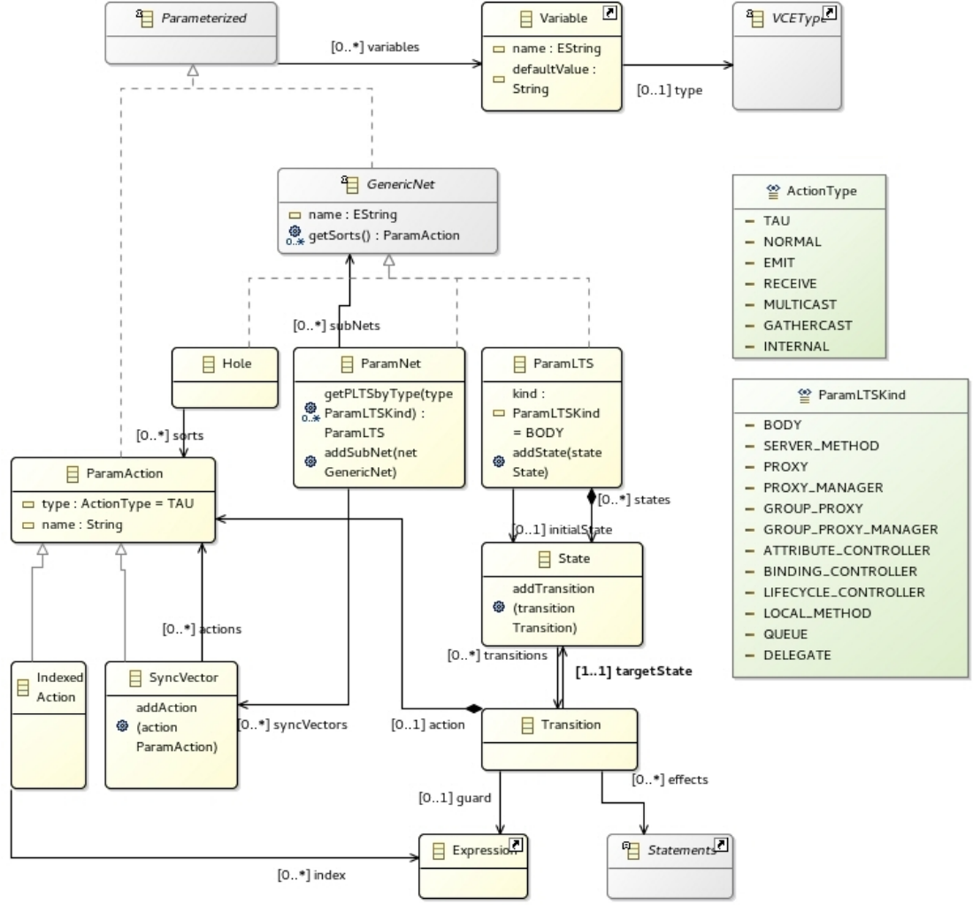
Figure 5.9 – pNets meta-model (simplified)
