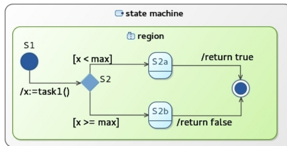
Figure 2.5 – UML state machine diagram
