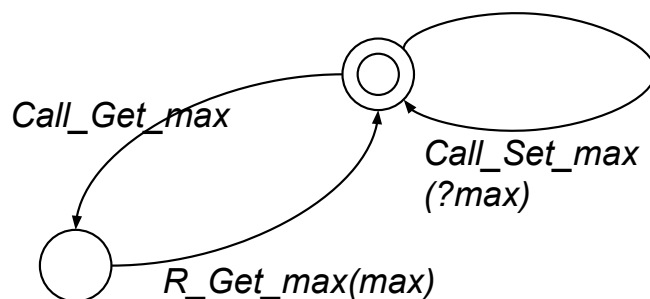
Figure 6.4 – An attribute controller pLTS
