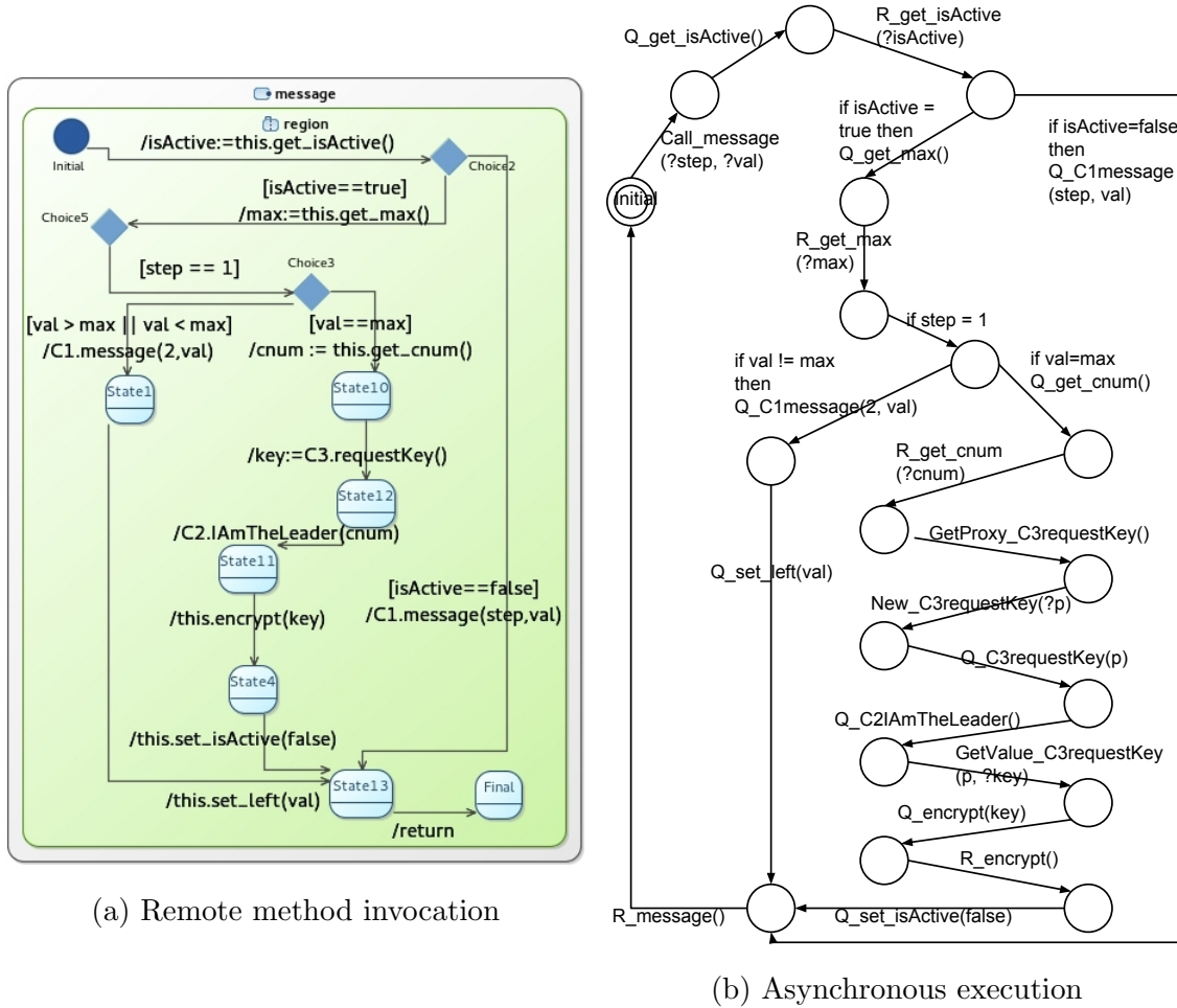
Figure 5.5 – A state machine and its translation to a pLTS
