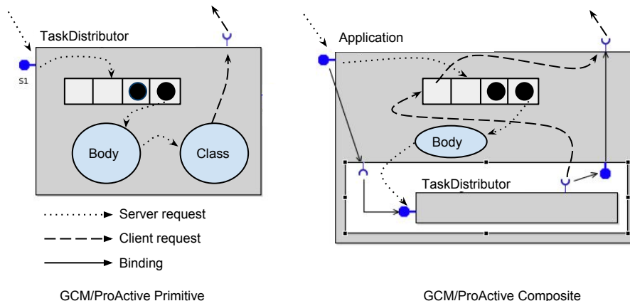
Figure 2.3 – Request treatment by GCM/ProActive components
