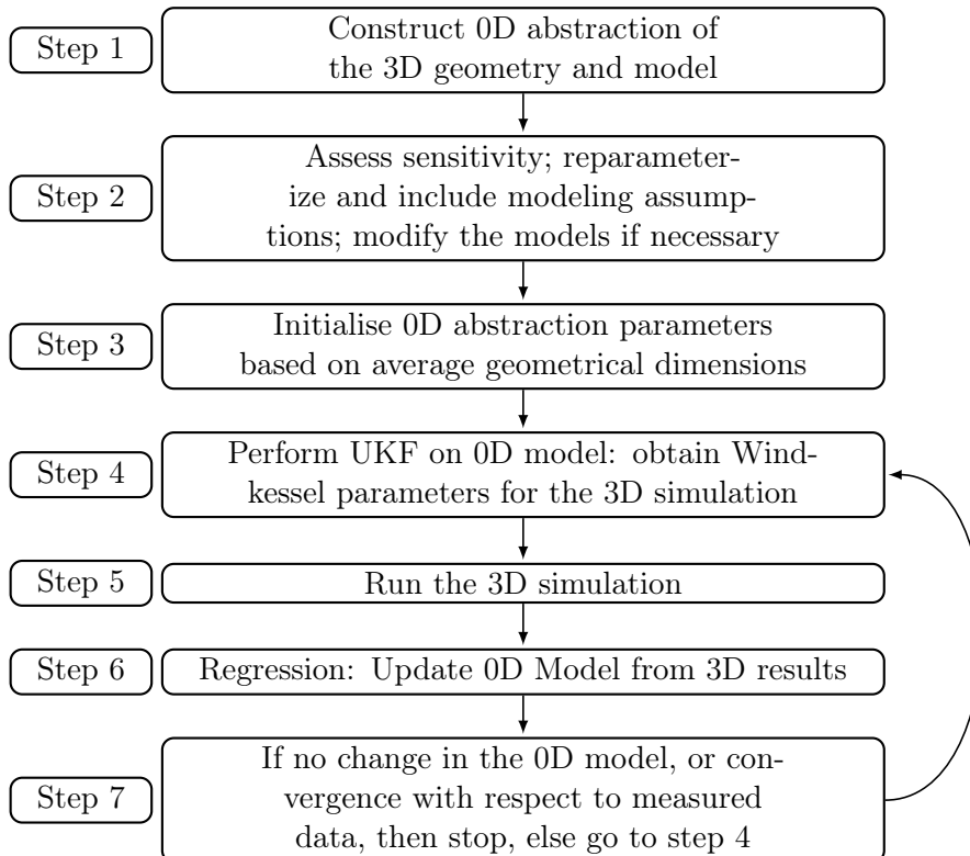
Figure 4.14: Algorithm for multidomain 3D simulations using sequential parameter estimation in a 0D model.
