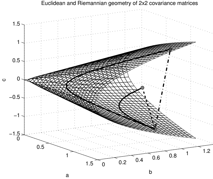
Figure 1.2: Comparison between Euclidean ( \delta_e - straight dashed lines) and Riemannian ( \delta_r - curved solid lines) distances measured between points of the space \mathcal{P}_2 .
