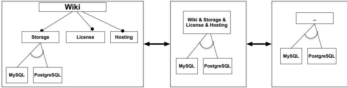
Figure 7.9: Logical feature groups: bi-implied features, clique contraction, parent place-holder
