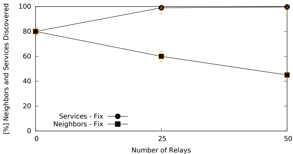
FIGURE 4.11: CACHACA - Number of Relays vs. Service and Neighbor Discovered (FIT IoT-lab).
