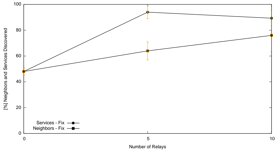
FIGURE 4.10: CACHACA - Number of Relays vs. Service and Neighbor Discovered (FIT IoT-lab).
