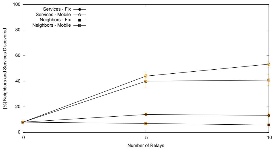
FIGURE 4.8: CACHACA - Number of Relays vs. Services and Neighbors Discovered.
