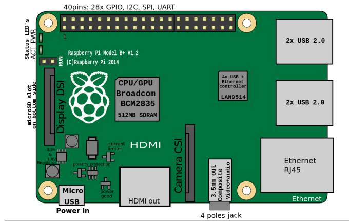
FIGURE 5.5: Raspberry Pi 2 - Model B. (source http://wikimedia.org )
