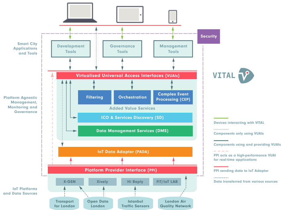
FIGURE 3.4: VITAL-OS architecture.
