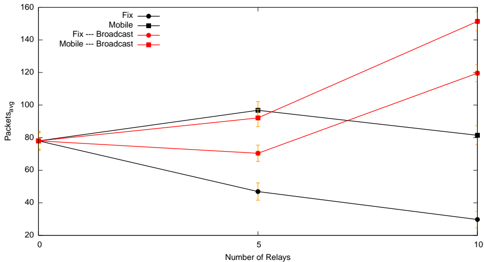
FIGURE 4.7: CACHACA - Number of Relays vs. Packet_{avg} sent.
