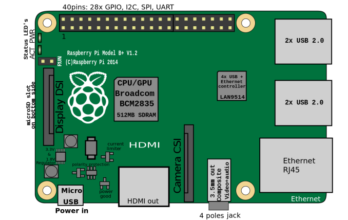
FIGURE 5.5: Raspberry Pi 2 - Model B. (source http://wikimedia.org )
