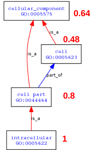
Figure 5.3: Semantic contributions of the ancestors of GO:0005622; here SV(GO:0005622) = 2.92 .
