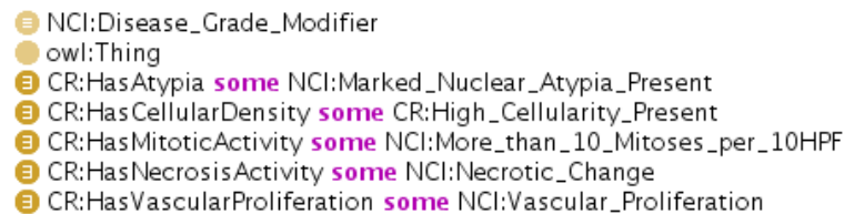
Figure 4.3: The Tumor10 from the evaluation set is defined according to its characteristics.
