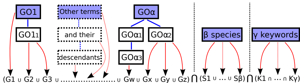
Figure 2.14: GO2PUB Query composition process using the parameters provided by the user. (1) the initial \alpha GO terms (purple boxes) are enriched by their descendants. (2) the genes (here noted G1 to Gz) annotated by the GO terms are retrieved. (3) the query is composed using the names, symbols and synonyms of the genes, the \beta species (S) and the \gamma MeSH or free keywords (K).
