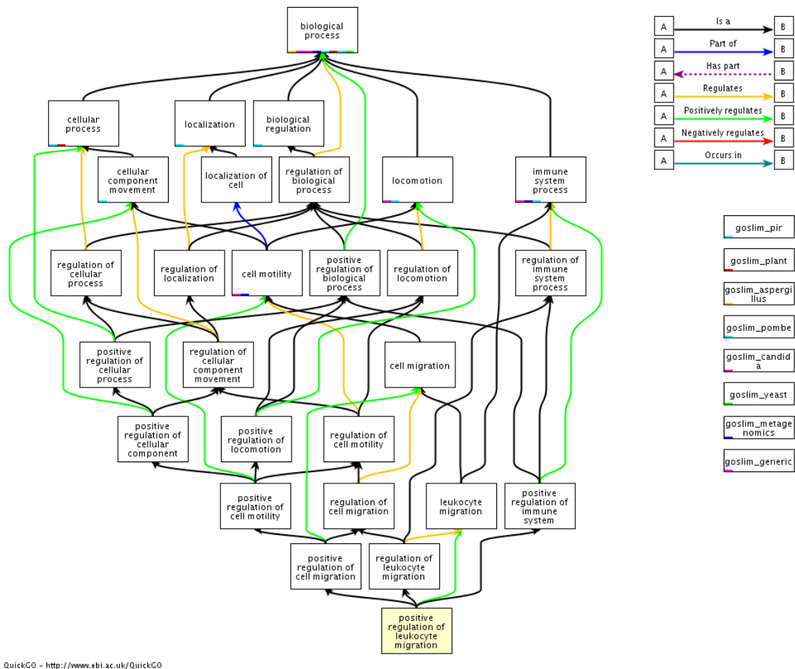
Figure 2.6: Complex mix of rdfs:subClassOf hierarchies and of rdfs:subPropertyOf hierarchies based on regulates , positively regulates and negatively regulates associating the GO class Positive regulation of leukocyte migration and its ancestors to the GO class Leukocyte migration and its ancestors (Image by QuickGO http://www.ebi.ac.uk/QuickGO/ ).
