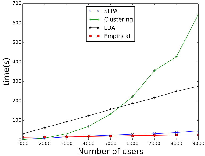
Figure 5.7: Scalability of the compared user interest detection methods
