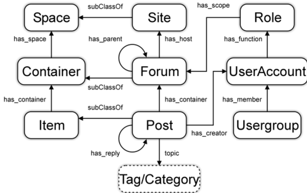
Figure 2.6: Overview of the SIOC ontology 20
