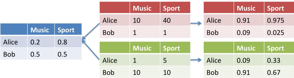
Figure 4.2: Different ways to estimate probabilities with topic assignment counts. The upper table: per-user topic distribution; the bottom table: per-topic user distribution
