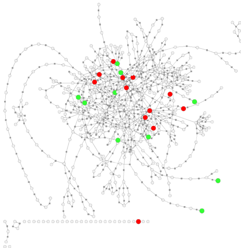
Figure 2.2: Yeast network. In red, the metabolites with a decreased concentration in the cadmium exposure condition. In green, the ones with an increased concentration in the cadmium exposure condition. Bottom left: disconnected compounds and reactions, including pyrroline-hydroxy-carboxylate. The squares represent the reactions and the circles represent the metabolites.
