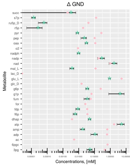
(a) Results obtained using the model provided in comparison to the results sent by the authors that were obtained at the time of their publication.
