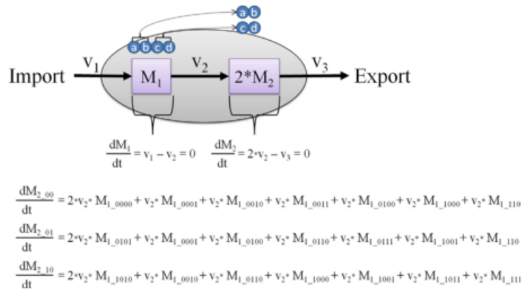
Figure 1.4: Figure from (Dersch et al., 2015). Different ways of modelling the metabolism. A) Topological: the focus is on the conversion of a metabolite (called substrate) to another metabolite (called product). B) Quantitative: the information is not only the transformation of M1 into M2 (with v_2 ), but also the quantities required, that is the stoichiometry. One mole of M1 will create 2 moles of M2. C) Steady-state metabolite balancing: here, an important hypothesis is added, which is that no metabolite is accumulated nor depleted. D) Dynamic metabolic balancing: using kinetic laws and parameters, variations in concentration and reaction fluxes along time can be inferred. E) Metabolic and isotopomer balancing: here, under the steady-state condition, it is possible to infer intracellular fluxes precisely using ^{13}\text{C} labelled substrate.
