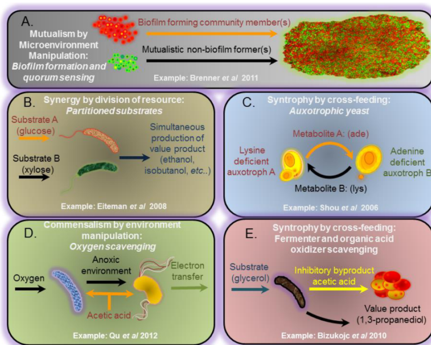
Figure 1.11: From (Bernstein and Carlson, 2012), different types of interactions that can occur in consortia (artificial or natural).
