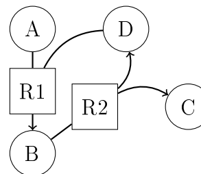
(e) Bipartite representation
