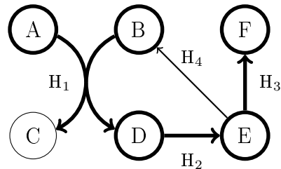
(b) The hyperpath \Pi_{S=\{A,B\}, t=F} is shown in bold. Both A and B are required for H_1 to be part of the path in the Definition 3.
