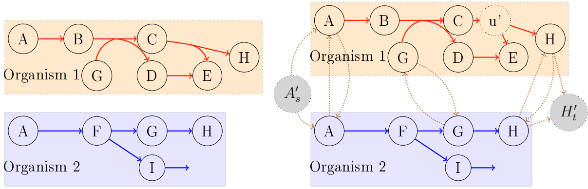
(a) Original networks, the two coloured squares represent two different organisms.
