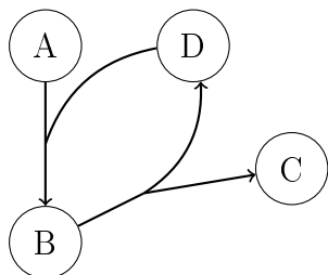
(d) Directed hypergraph representation
