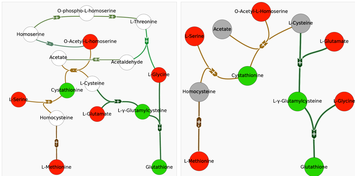
(a) Solution when all vertices are considered (no isolated grey vertices). (b) Solution with grey vertices. The number of hyperarcs and of isolated grey vertices is minimised.
