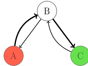
(b) Here, the directed hypergraph of Figure 2.9a was transformed. In bold, the solution meets Definition 9. B is not a source not a sink whereas A is a source and C is a sink.
