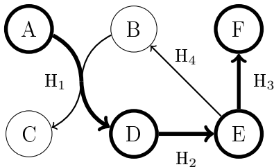
(a) The hyperpath \mathcal{P}_{A,F} is shown in bold, it is possible to reach F only with the starting vertex A using Definition 2.
