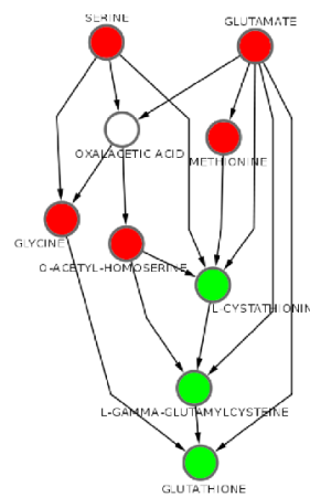
(c) A story
