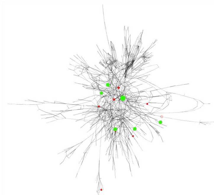
(a) Original network.
