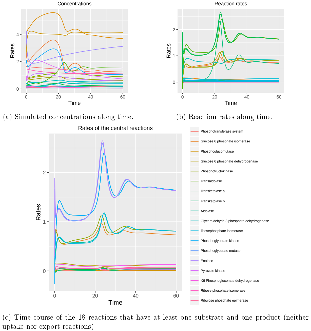
Figure 3.6: Results of the time-course simulations.
