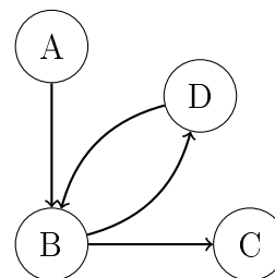
(c) Compound digraph representation
