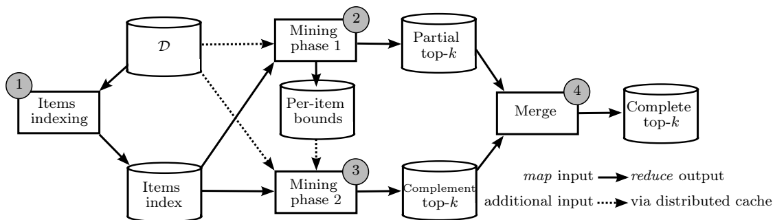
Figure 4.5: Hadoop implementation of TOPPI
