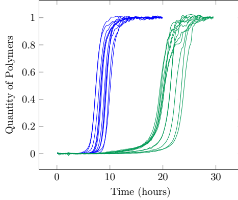
Figure 2.2: Twelve experimental timecourse of polymerised mass for two given initial concentrations of monomers: 122 \mu M (blue) and 30.5 \mu M (green) published in [Xue et al., 2008].
