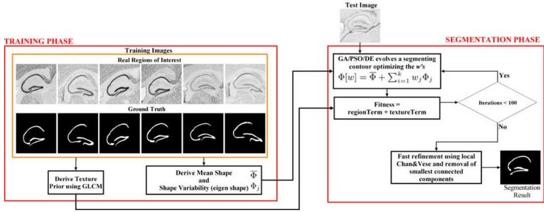
Figure 6.1: General Overview of the Hippocampus Segmentation System
