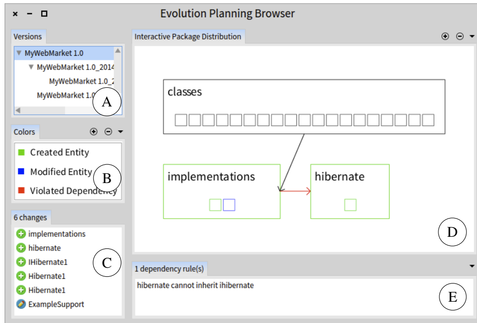
Figure 3.1: ORIONPLANNING overview.
