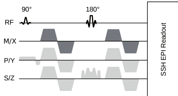
Figure 1.1: DTI spin echo pulse sequence with single shot EPI readout. Diffusion encoding is established with a pair of velocity compensating bipolar gradients. For local look imaging, the excitation pulse is applied in phase encoding direction, while the echo pulse remains in slice-select direction. The echo pulse duration is shortened using VERSE.
