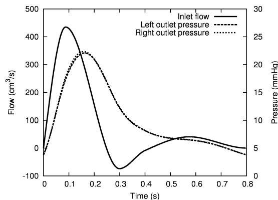
Figure 8.8: Normal boundary conditions: flow rate is prescribed at the inlet (with a mean value of 4.9 \text{ L} \cdot \text{min}^{-1} ) and outlet pressure for the atlas obtained the Windkessel model in Table 8.1. These outlet pressures change slightly from one geometry to another.
