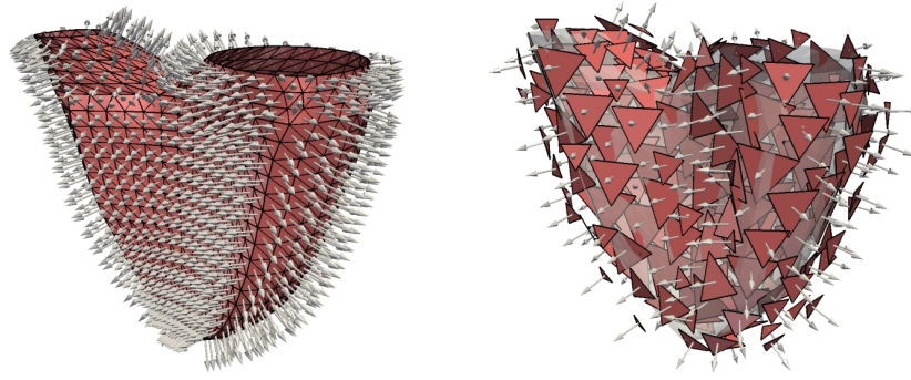
Figure 4.3: The Dirac delta currents of a triangulated mesh are the normal vectors of every face, centred at the face barycentre. A greedy algorithm reduces the amount of delta currents needed to represent the shape while preserving the accuracy of the representation.
