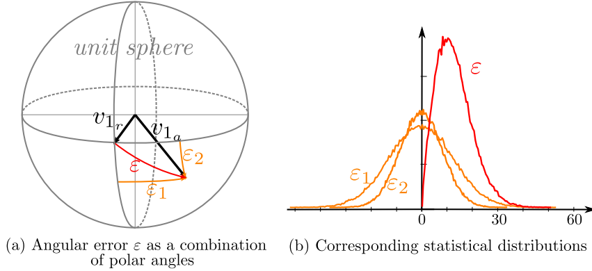
Figure 1.12: (a) Residual error \varepsilon due to the approximation scheme on the angle between the approximated tensor's first eigenvector v_{1_a} and that of the reference tensor v_{1_r} . \varepsilon can be seen as a combination of two independent polar signed angles \varepsilon_1 and \varepsilon_2 . (b) If \varepsilon_1 and \varepsilon_2 have a zero-mean Gaussian distribution, then the distribution of \varepsilon is strongly skewed, and depends on the standard deviations of the polar angle errors.
