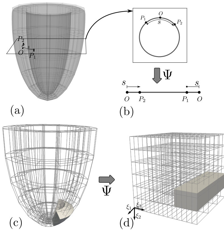
Figure 1.4: (a,b): A short axis circle drawn in the Cartesian space (a) is represented as a segment in the Prolate Spheroidal (PS) frame (b). \xi_3 being defined with a modulo, the segment is reproduced at infinity on both sides, and the barycentre of P_1 and P_2 remains O . (c,d): A left ventricle volume is non convex in a Cartesian frame (c) whereas the same volume expressed in a PS frame becomes a convex box (d).
