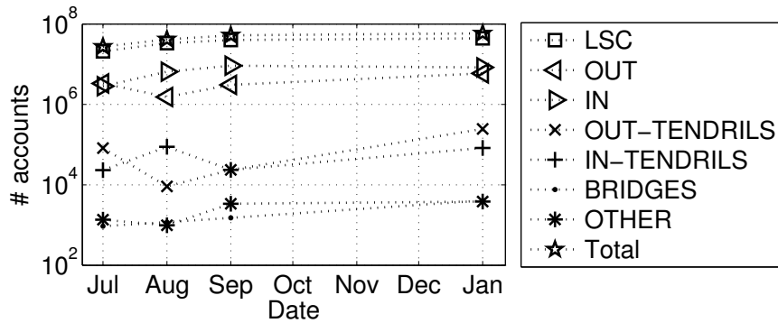
Figure 3.8 – Comparison of our estimated graphs of 2009 (labeled Jul and Jan) with two existing Twitter datasets made in August [Kwak 2010] and September [Cha 2010] 2009. Our simple methodology gives an approximation of the macrostructure of the Twitter social graph that is consistent with existing datasets.
