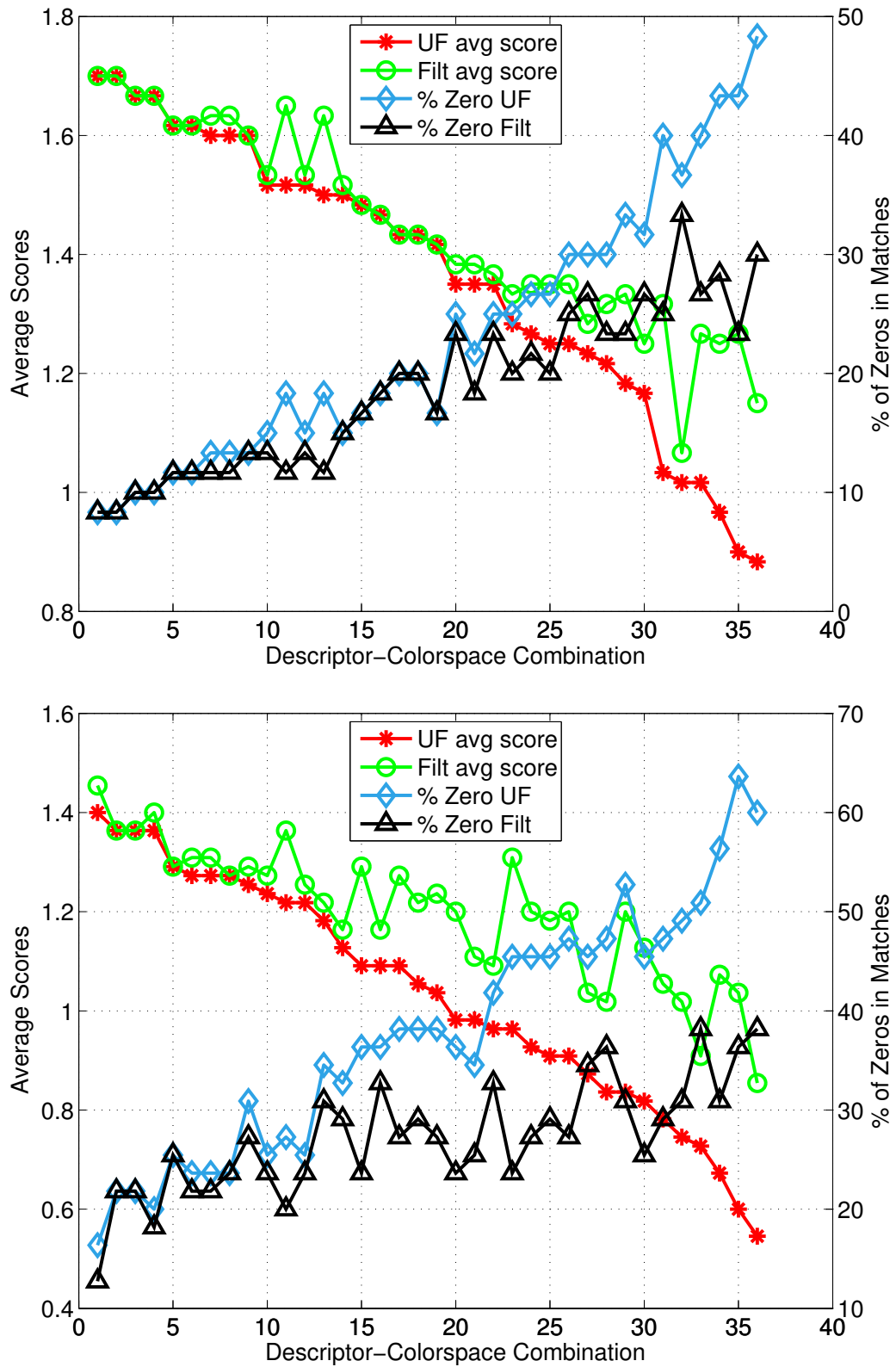
Figure 7.10: Avg. scores on the left axis and % of images matched with score zero on the right axis for all 36 of the descriptor-colorspace combinations. The x-axis is sorted by the best avg. score. NBI ( top ) and WL ( bottom ).
