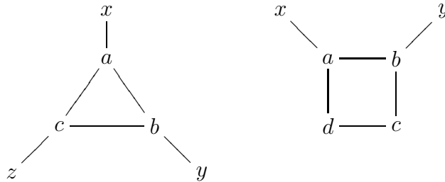
Figure 7.4.1: The graphs 3C and AC.
