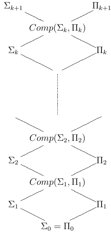
Figure 0.2.1: The alternation-depth hierarchy
