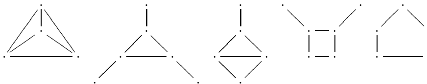
Figure 6.4.1: The minimal and complete excluded minors characterizing the undirected graphs of entanglement at most 2.
