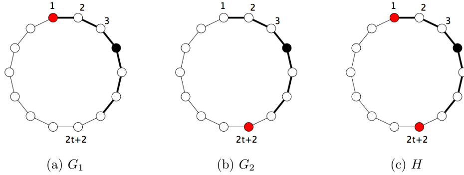
Figure 2-2: Illustration of Leader \notin LD for t = 3 . Red nodes are leaders. The black node has the same view in H as in G_1 . Since \mathcal{A} is correct for G_1 , the black node outputs yes in H . The same goes for all other nodes.
