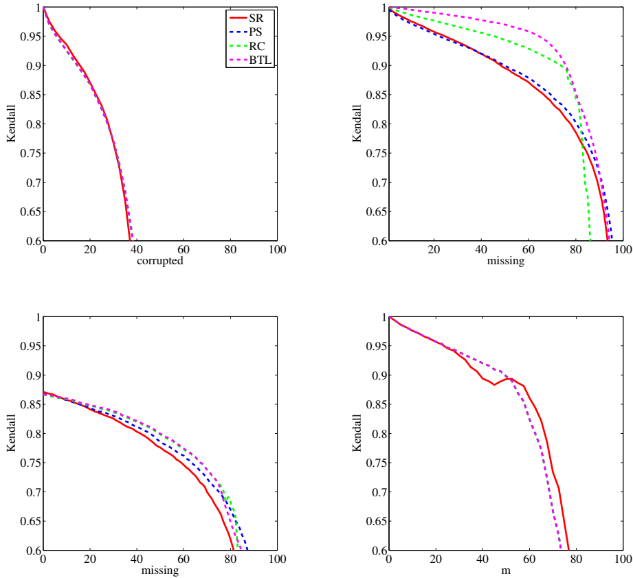
FIGURE 4.5: Kendall \tau (higher is better) for SerialRank with normalized Laplacian (SR, full red line), row-sum (PS, ( Wauthier et al., 2013 ) dashed blue line), rank centrality (RC ( Negahban et al., 2012 ) dashed green line), and maximum likelihood (BTL ( Bradley and Terry, 1952 ), dashed magenta line). In the first synthetic dataset, we vary the proportion of corrupted comparisons ( top left ), the proportion of observed comparisons ( top right ) and the proportion of observed comparisons, with 20% of comparisons being corrupted ( bottom left ). We also vary the parameter m in the second synthetic dataset ( bottom right ).
