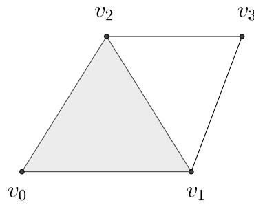
Figure 7.3: 2-dimensional simplicial complex.
