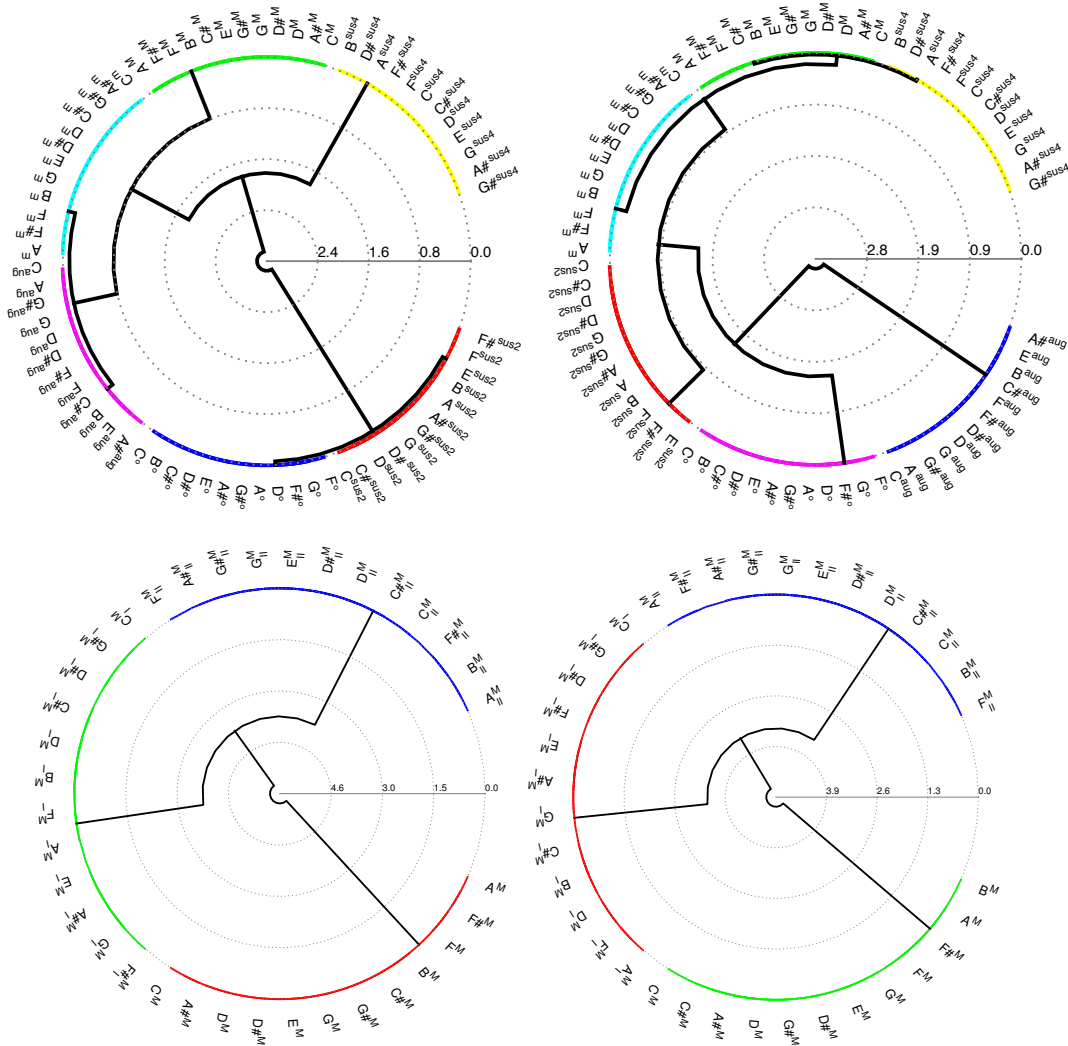
Figure 9.10: Hierarchical structure of triads' consonance. In the first row it is possible to observe how the consonance classifies triads according to their classes, by using two different harmonic spectra. In the second row the inversions of the major triads are classified according to their consonance value, computed with h_1 and h_2 , respectively.
