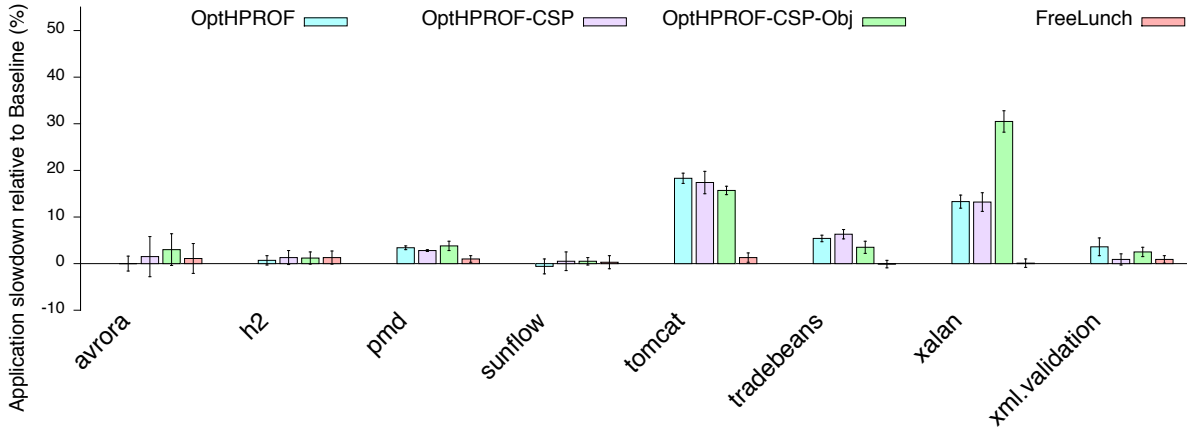
Figure 4.2: Overhead on execution time compared to baseline.
