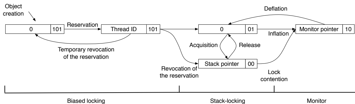
Figure 2.4: State-transition diagram of the mark word between lock algorithms.
