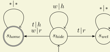
Figure 40 – The game Hide-or-Run : \mathbb{G}_{HR}
