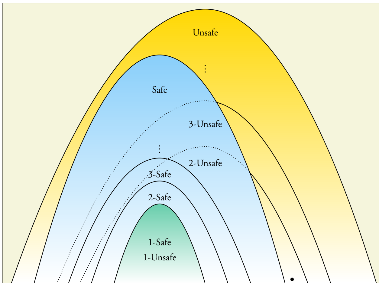
Figure 16 – The Safe/Unsafe hierarchies.
