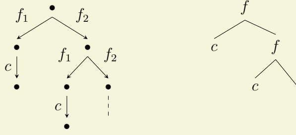
Figure 3 – Two representations of the infinite term f_2^* \{f_1 c, f_1, \varepsilon\} = f(c, f(c, f(\dots))) over the ranked alphabet \{f, c\} assuming that \varrho(f) = 2 and \varrho(c) = 0 .
