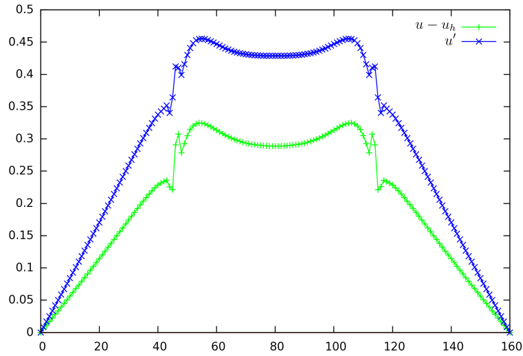
Figure 6.14: Thin bubble case: comparison of (+) error u - u_h and (x) Defect-Correction corrector.
