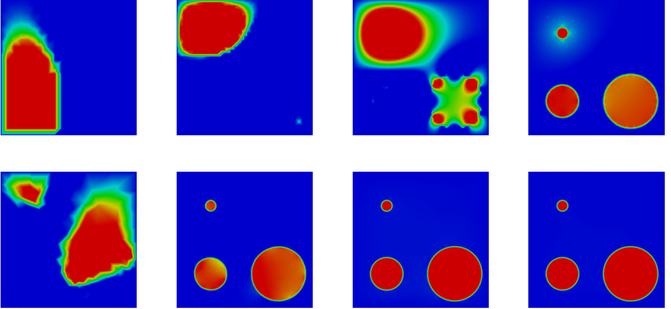
Figure 6.16: Multiple bubble test case: top: non-adaptive solutions for 441, 1681, 6561, 25921 nodes, and, bottom, the mesh adaptive solution for about the same number of nodes (palette restricted to values between the minimum (0.) and the maximum (1.) of the exact solution.
