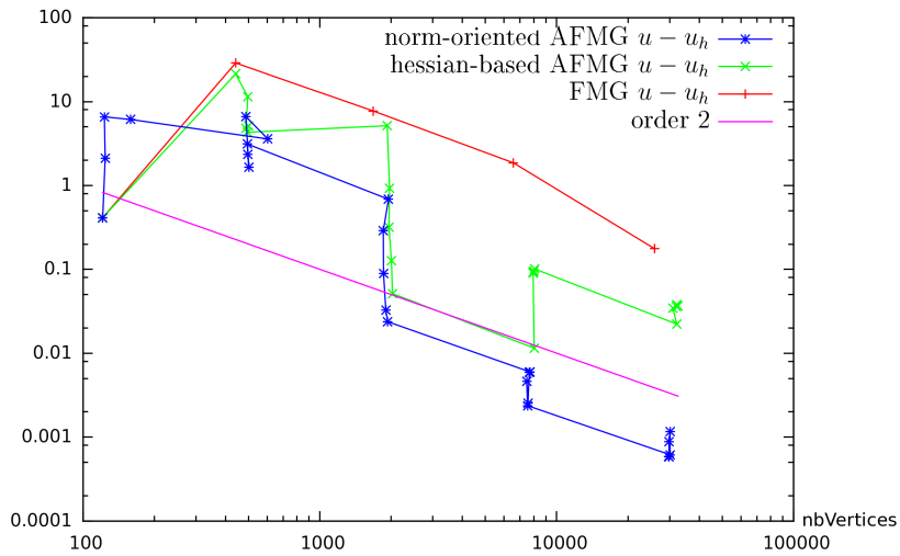
Figure 6.15: Thin bubble test case: convergence of the error norm |u - u_h|_{L^2} as a function of number of vertices in the mesh for (+) non-adaptative FMG, (x) Hessian-based adaptative FMG and (*) norm-oriented adaptative FMG.
