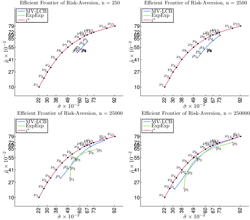
Figure 3.9: Risk tolerance sensitivity of MV-LCB and ExpExp for Configuration 1 .
