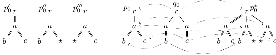
Figure 14 – Immediate anchored generalizations versus an embedding with overlap.
