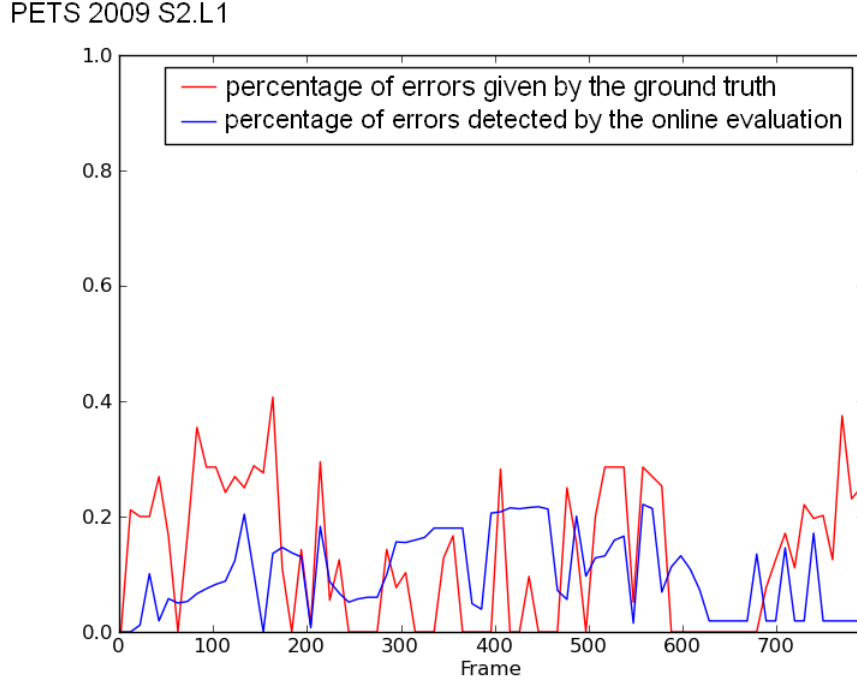
Figure 2.8: Comparison between the percentage of errors per frame given by the ground truth (red) and the percentage of errors found by the online evaluation (blue) on sequence S2.L1.View1 of PETS2009 using tracker 1
