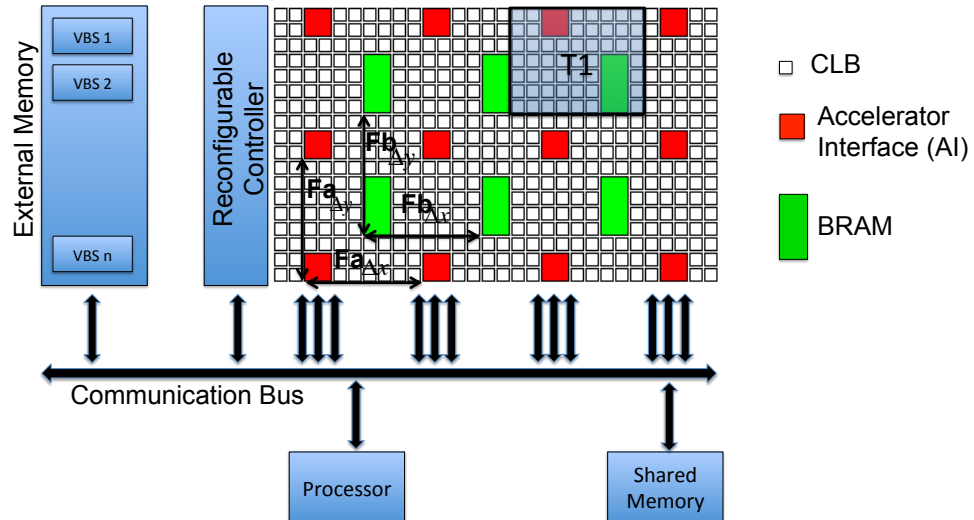
FIGURE 4.2: 2D Heterogenous FPGA
