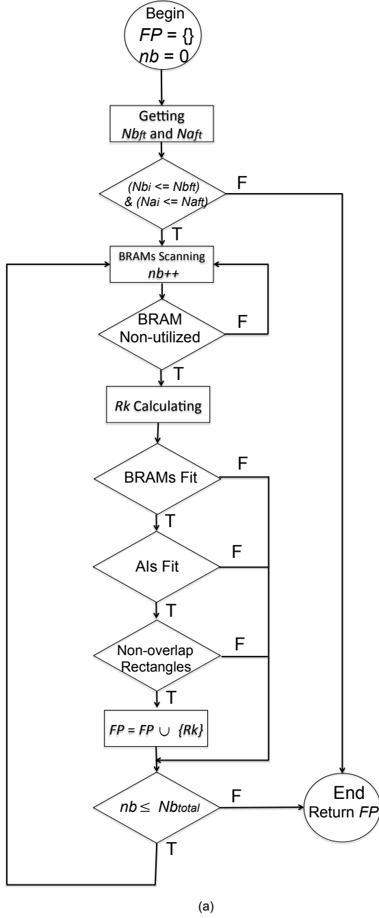
FIGURE 4.6: Quick search method for finding all feasible regions R_{k,i} for the task T_i at time t
