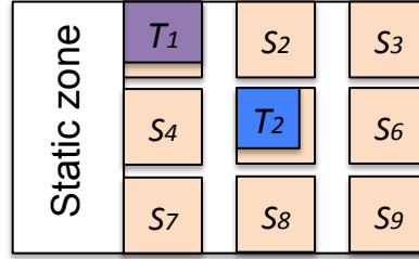
FIGURE 2.8: Reconfiguration by slot. T_1 is executed on S_1 and T_2 on S_5
