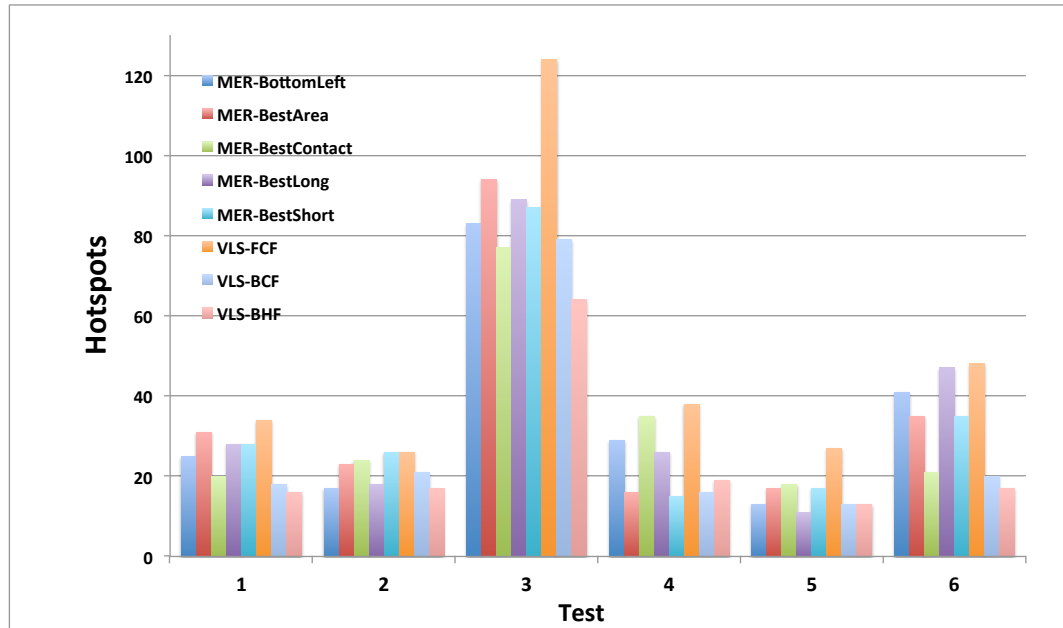
FIGURE 3.10: Comparisons of hotspots for different scheduling and placement techniques
