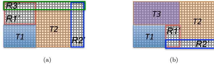
FIGURE 2.13: -a- The placement of T_2 creates the FPGA fragmentation and prevents T_3 not to be placed -b- The placement of T_2 creates a low FPGA fragmentation and allows T_3 to be placed
