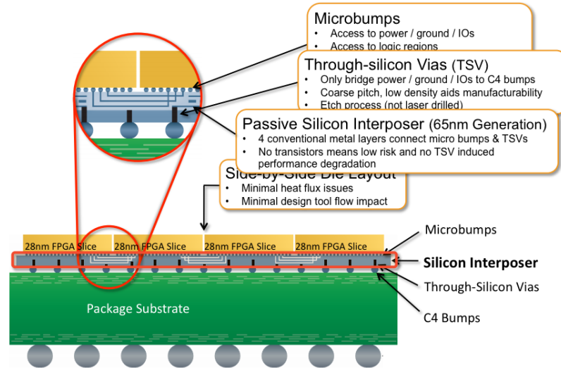
FIGURE 2.17: Virtex 7 - 2000T (figure taken from [2])
