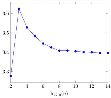
Figure 4.3: Average maximal size of the list divided by n^{1/3}
