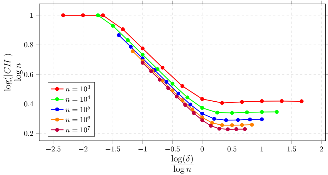
(a) Experimental results for the complexity of the convex hull of a \ell^\infty perturbation of amplitude \delta of the regular n -gon inscribed in the unit circle. Each data point corresponds to an average over 1000 experiments.
