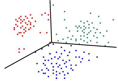
An example of clustering with k = 3
