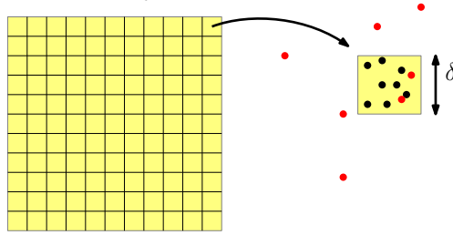
For each cell C_j , we consider the initial points in C_j (in black) and their noisy version (in red).
