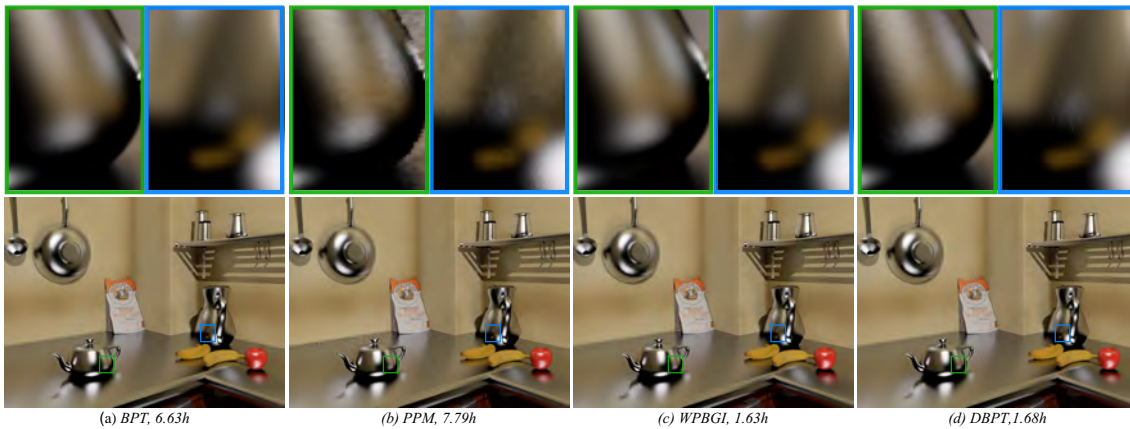
Figure 10 Corner scene comparison: Visual comparison of final renderings.
