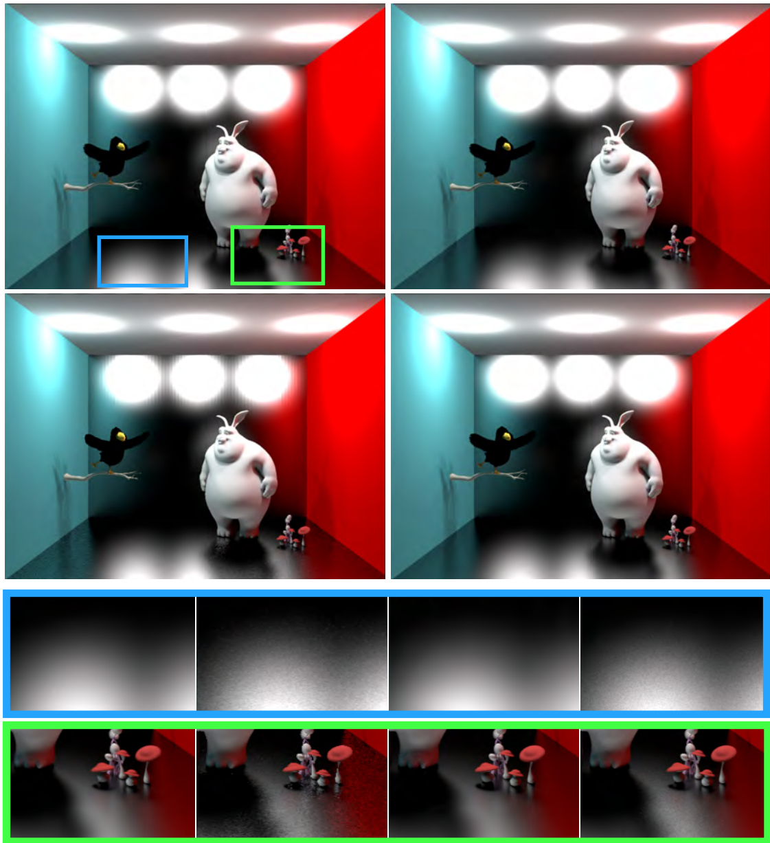
(a) BPT , 10.53h (b) PPM , 10.07h (c) WPBGI , 1.04h (d) DBPT , 1.33h
