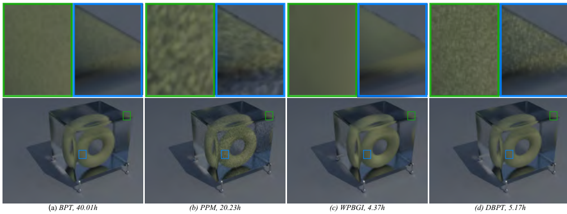
Figure 15 Torus scene comparison.
