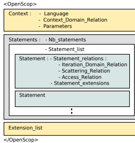
Figure 2.6 – OpenScop Data Structure .
