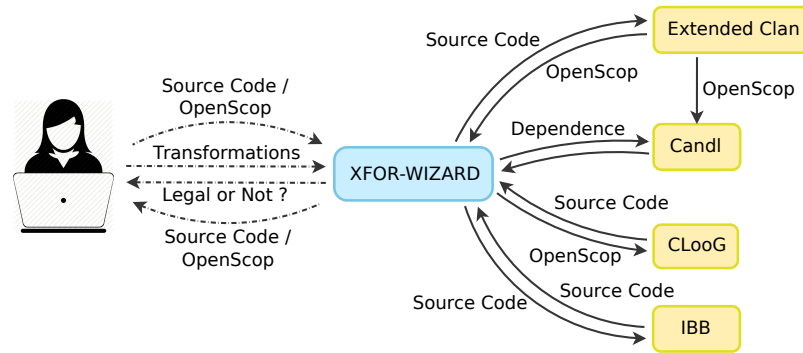
Figure 7.5 – XFOR-WIZARD Architecture and Interactions.
