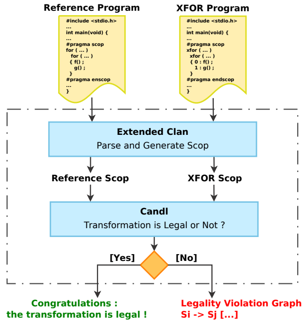
Figure 7.1 – XFORSKAN Architecture.
