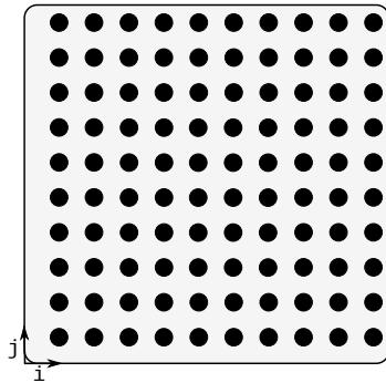
Figure 4.3 – First Domain.
