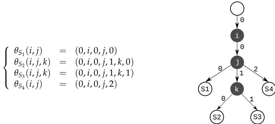
Figure 2.3 – Abstract Syntax Tree.
