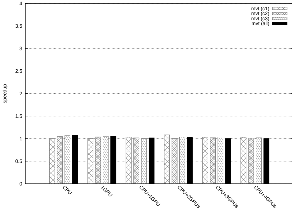
Figure 5.31 – Speedup to execution time of slowest code version combination for mvt .
