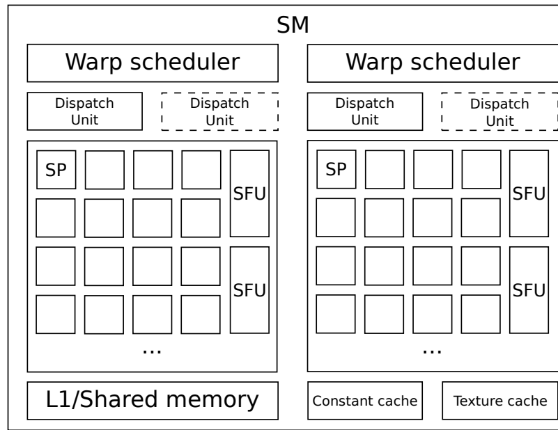
Figure 3.3 – Insight of a Streaming Multiprocessor (SM) organization.
