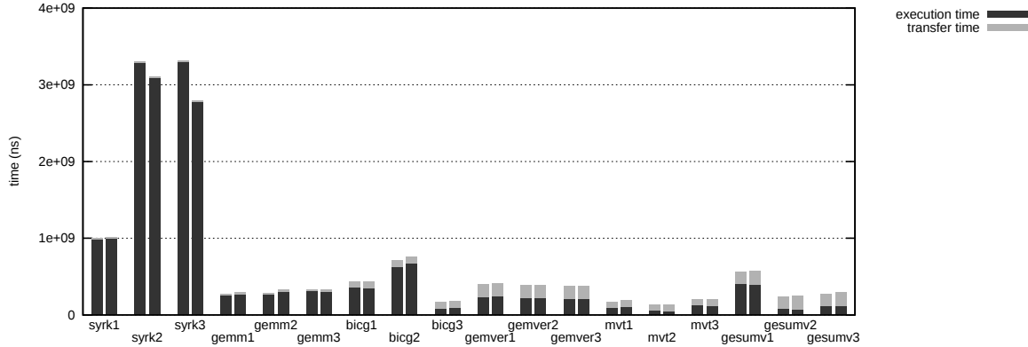
Figure 4.17 – Comparison between prediction (left bar) and real (right bar) execution times on PolyBench with large dataset on GTX680.
