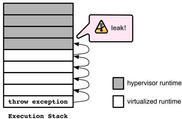
Figure 4.7: Reference Leaks in a Mixed Stack on Exception. When mixing the execution stack between the virtualized and hypervisor runtimes, an exception may traverse the stack and have access to a reference from a different application runtime.
