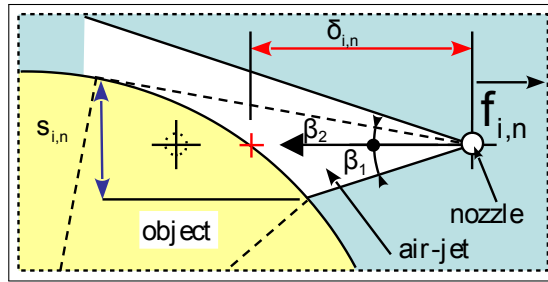
Figure 7.8: Model of one Air-jet
