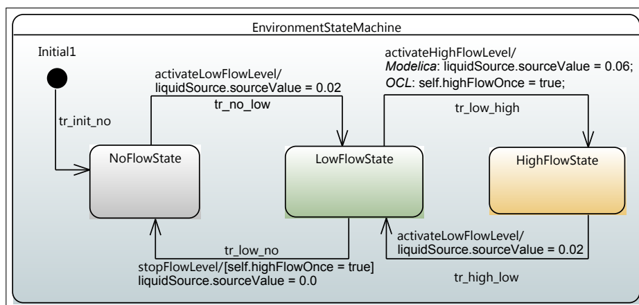
Figure 5.6: State Machine of the Environment
