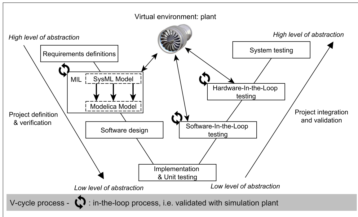
Figure 2.1: V-cycle Process Starting with SysML Model
