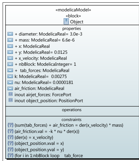
Figure 7.4: SysML Block of the Object
