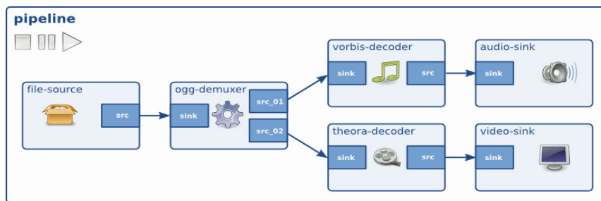
FIGURE 2.5 – Application multimédia reposant sur un pipeline GStreamer [GS15]
